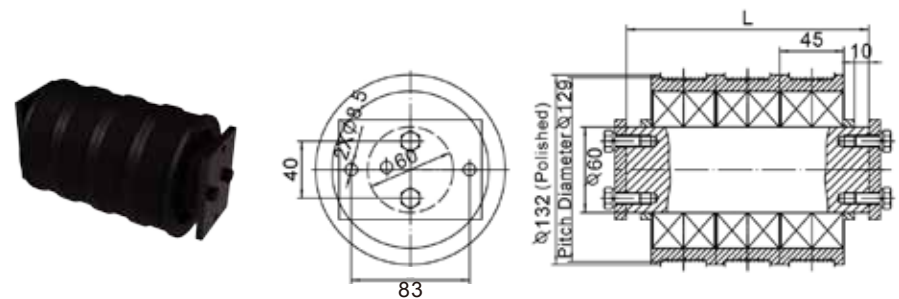
Counter Pulley Set - 132 Series
